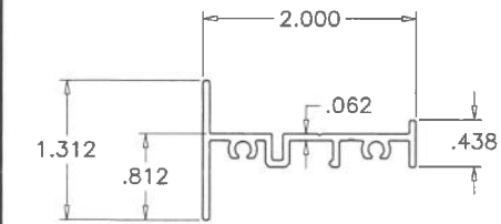
1 WINDOW FRAME
