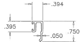
2 GLZING BEAD
