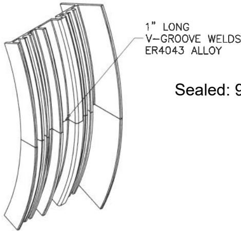
CIRCULAR WINDOWS
